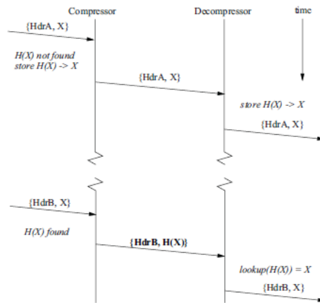
Figure 4: Compression protocol
